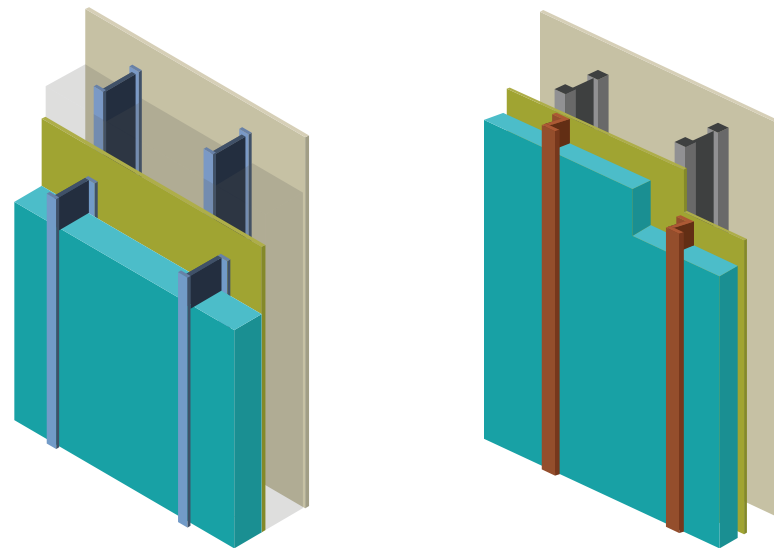
Wall assembly using vertical steel girts
