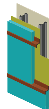
Wall assembly using horizontal ArmaGirt™ Z-Girt
