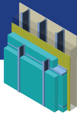
VERTICAL & HORIZONTAL ARMAGIRT™ Z-GIRT
