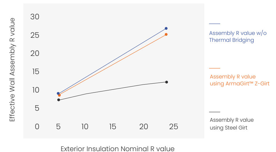
EFFECTIVE WALL ASSEMBLY R VALUE COMPARISON WITH HORIZONTAL GIRTS AT 24" SPACING
