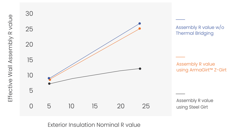
EFFECTIVE WALL ASSEMBLY R VALUE COMPARISON WITH VERTICAL GIRTS AT 16" SPACING
