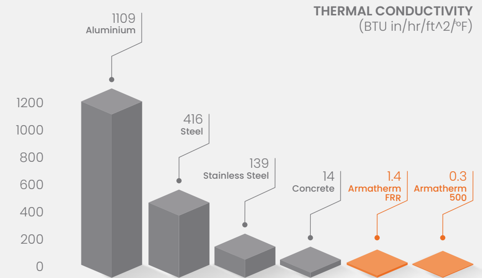
Thermal conductivity values of Armatherm structural thermal break materials as compared to standard building materials.
